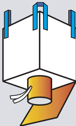
Discharge Spout w/ Flap
