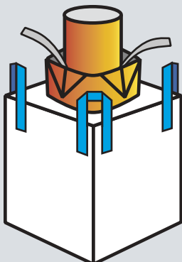
Fill Spout w/ Petal Closure
