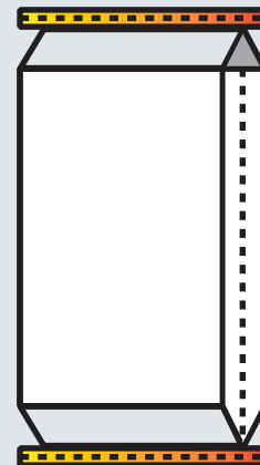
V-G-SB Valve - Gussetted Sewn Bottom
